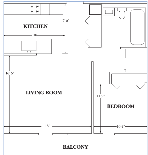
Floor plan of a typical 560-square-foot apartment
