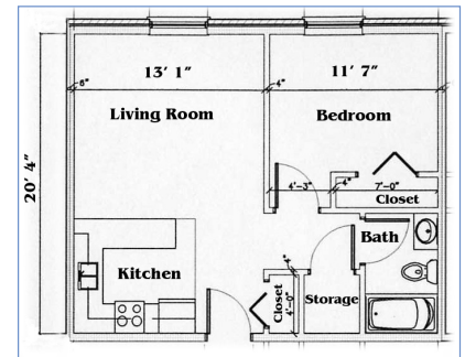
Floor plan of a typical unit
